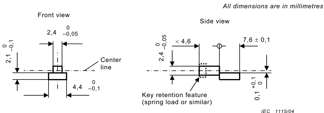
Figure 5 – Key dimensions
