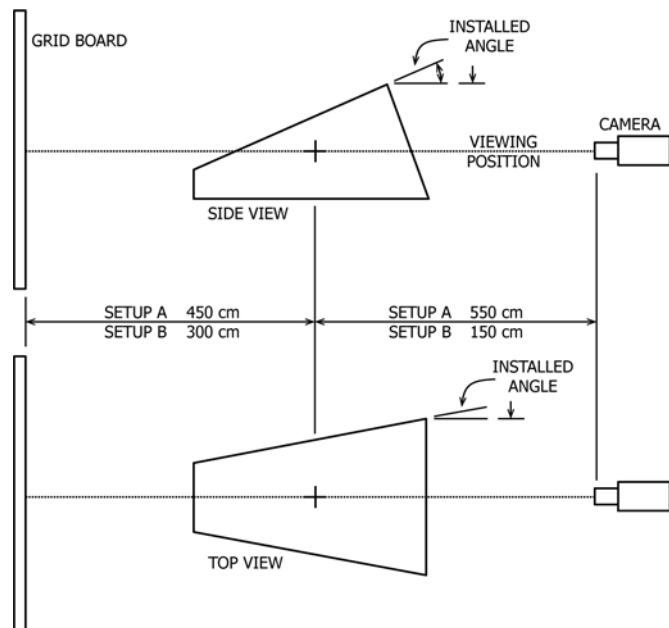
FIG. 2 Schematic Diagrams of GLS Photographic Recording Distances
