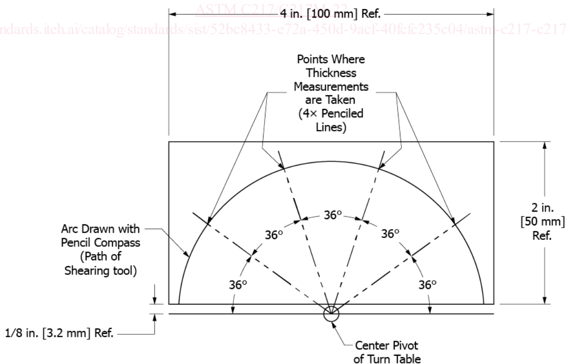
FIG. 2 Diagram of Slate Specimen Prepared for Test with Shear/Scratch Tester
