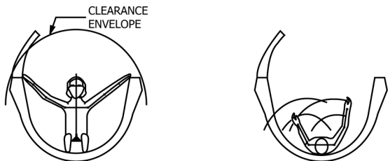
CHILDREN'S CLEARANCE WITH RISERS
