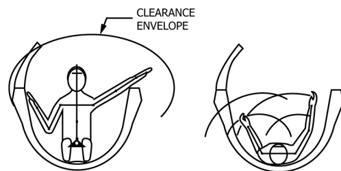
ADULTS CLEARANCE WITH RISERS
