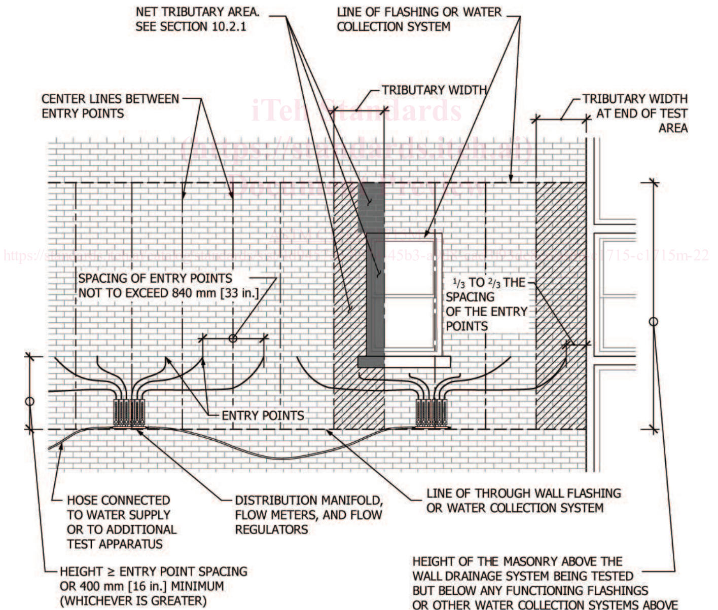
FIG. 5 Elevation of Type 1 System
