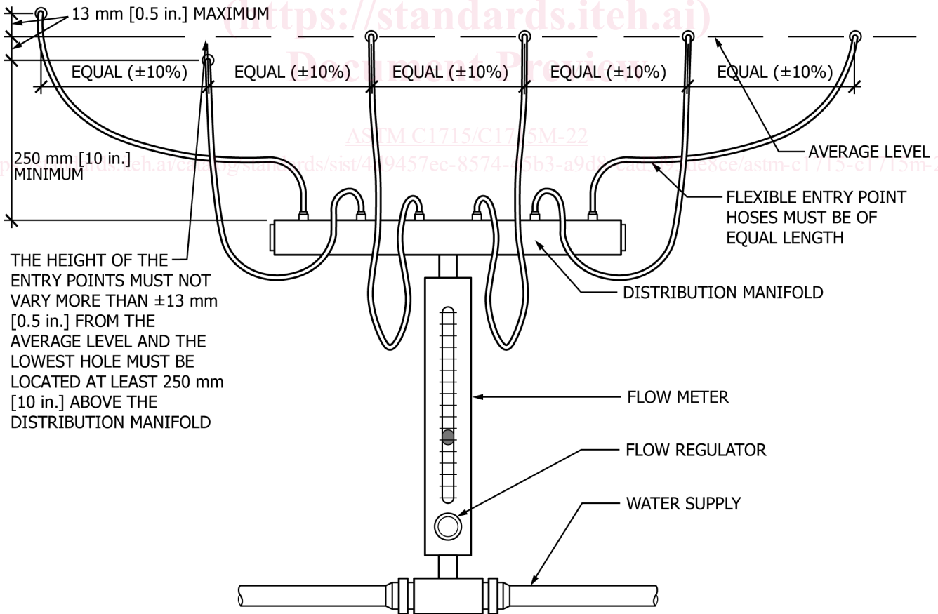
FIG. 2 Flow Meter Connected to Multiple Entry Points (Type 2)
