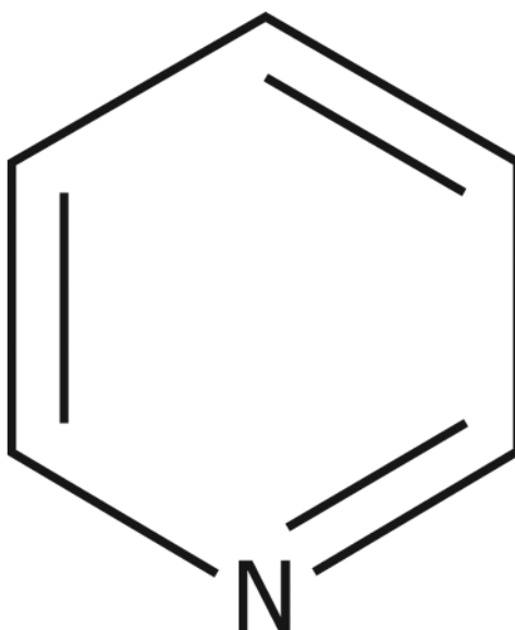
FIG. 1 Pyridine CAS [68391-11-7]
