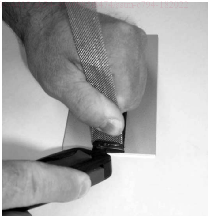
FIG. 9 Cut Along Sealant/Substrate Interface with Razor Knife
