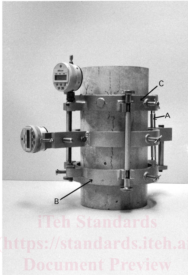
FIG. 1 Suitable Compressometer
