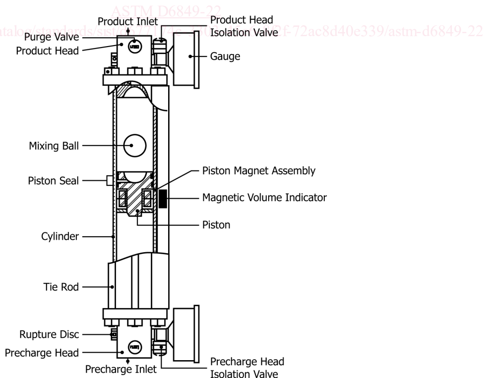
FIG. 1 Typical Floating Piston Cylinder (FPC)
