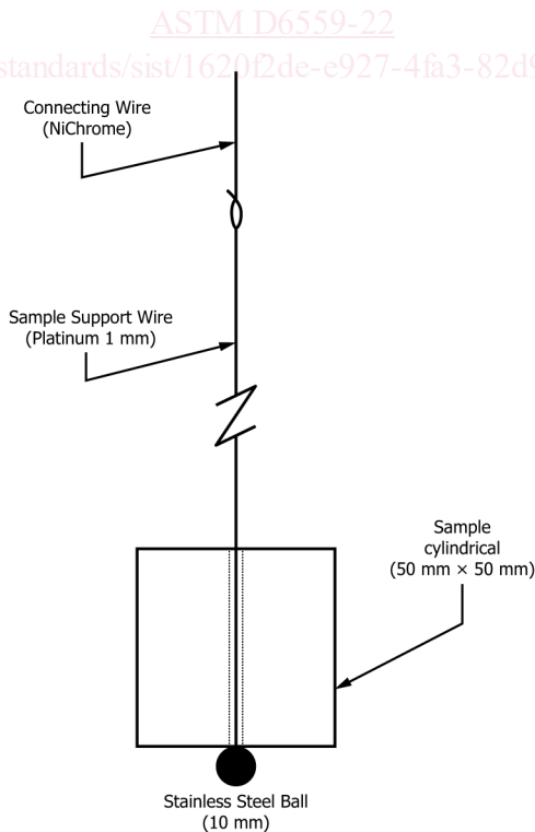
FIG. 2 Typical Sample Holder
