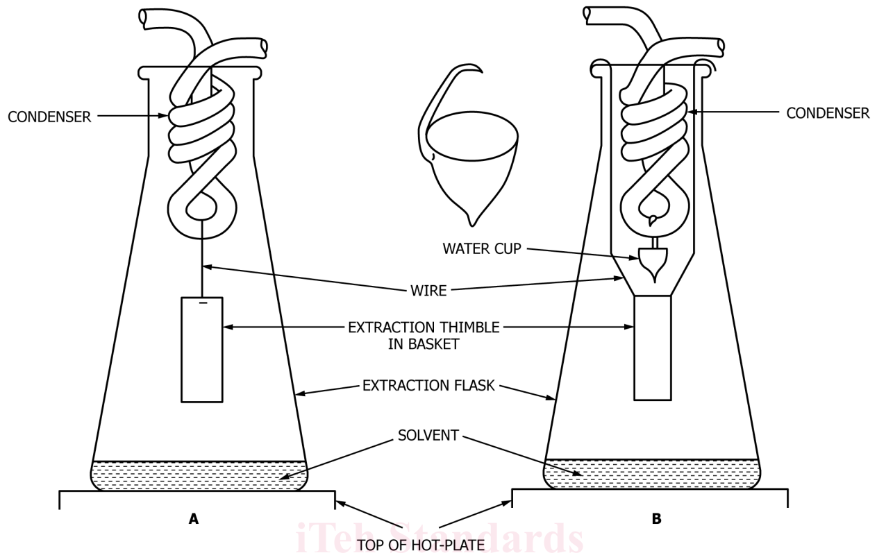
FIG. 1 Extraction Apparatus for Determination of Sediment
