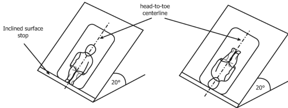
FIG. 10 CAMI Dummy Position when Product Short Side Touches the Inclined Surface Stop
