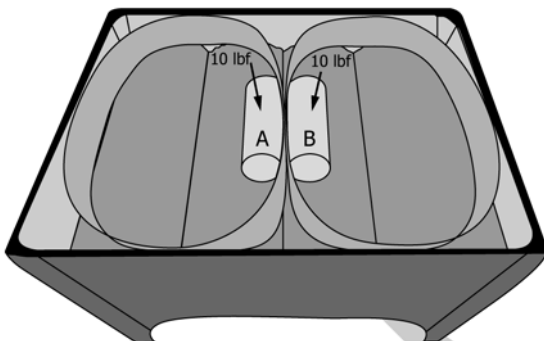
FIG. 20 Two Cylinders (A and B) in Contact with Inside Wall
