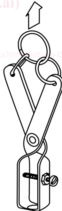
FIG. 11 Sketch of Clamping Device
