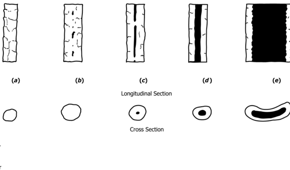
FIG. 1 Types of Medulla in Wool and Mohair Fibers
