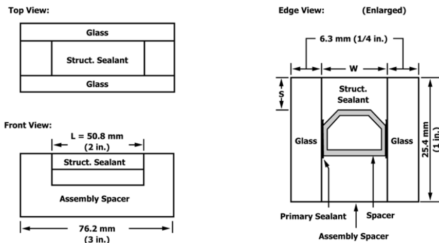
FIG. 2 Test Specimen
