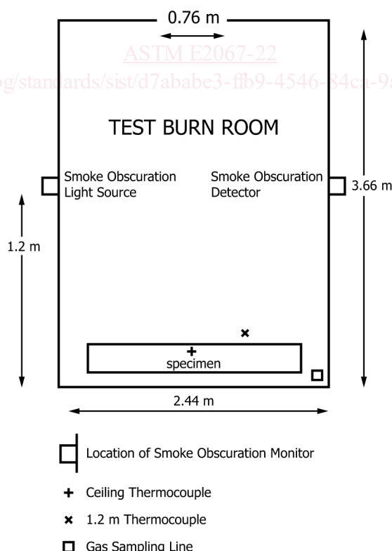
FIG. 1 Test Room Configuration A (ASTM room)
