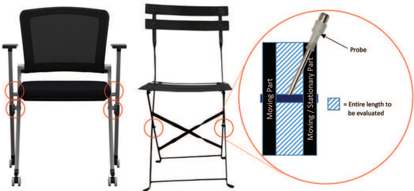
FIG. 1 Examples of Evaluation Between Moving Parts and Between Moving and Stationary Parts
