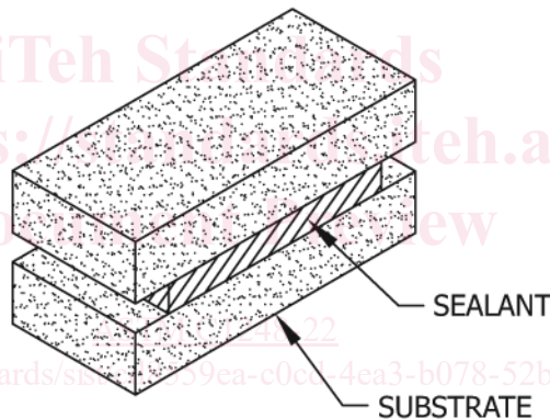
(B) SPECIMEN AFTER APPLICATION OF SEALANT & REMOVAL OF SPACER
