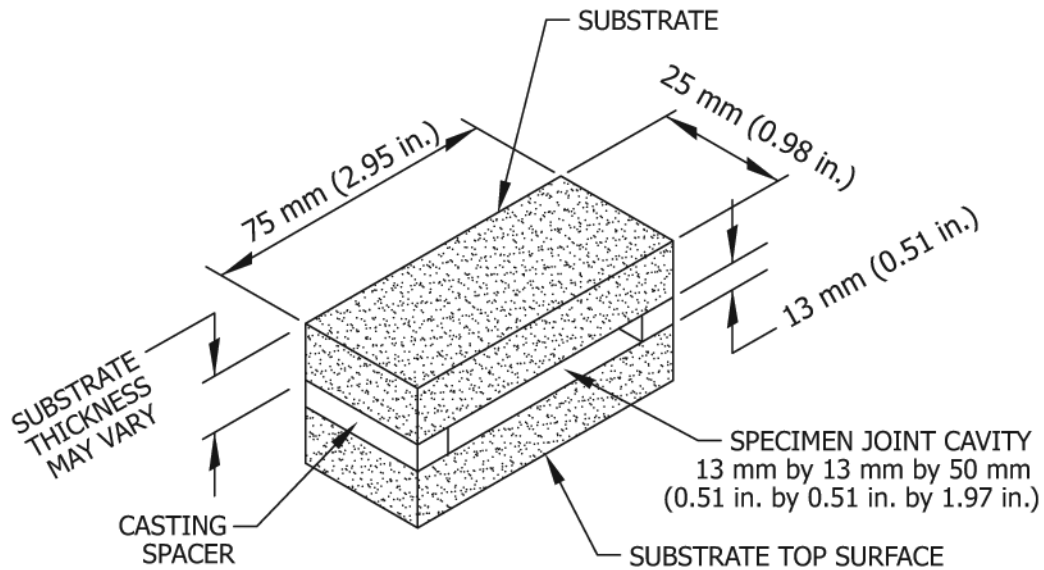
(A) PREPARED SPECIMEN BEFORE APPLICATION OF SEALANT
