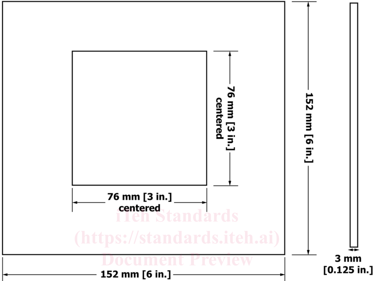
76 mm [3 in.] square hole centered in the middle of each of the 152 by 152 mm [6 by 6 in.] plates.
