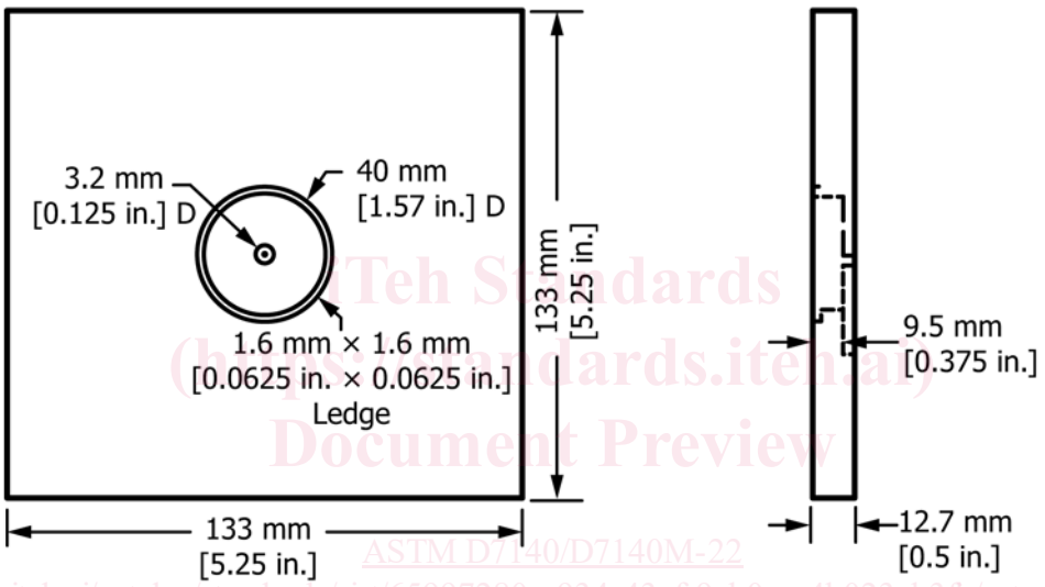
FIG. 2 Calorimeter Placement
