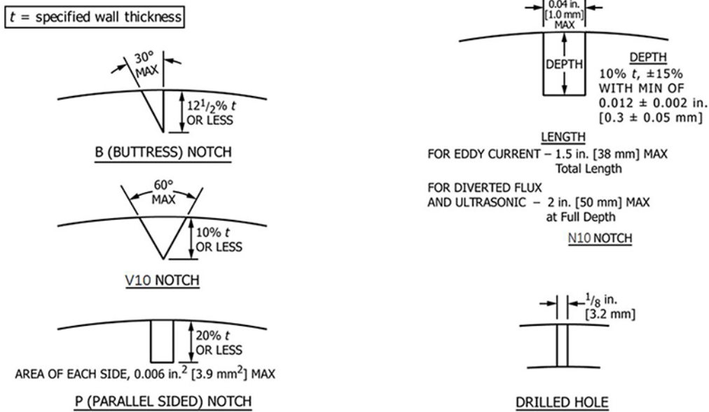
FIG. 1 Calibration Standards
