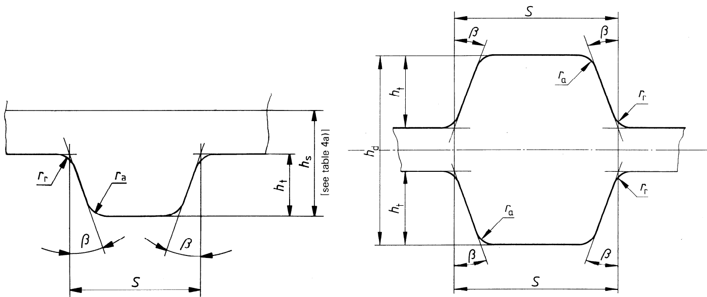
a) One-sided synchronous belt
