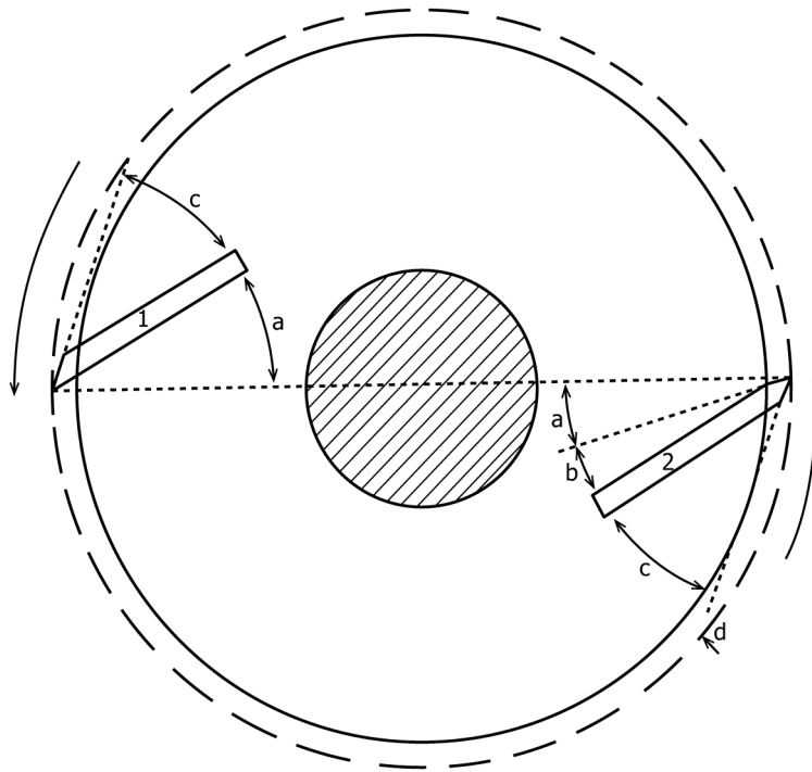
(a) Cutting angle. (c) Clearance bevel. (a) Cutting angle. (c) Clearance angle. (b) Cutting bevel. (d) Cutting circle.
