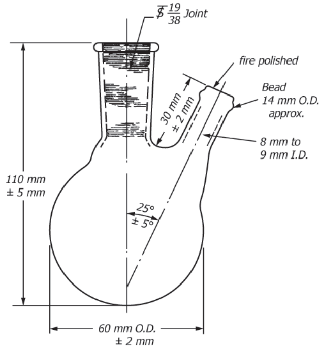
100 mL Flask
