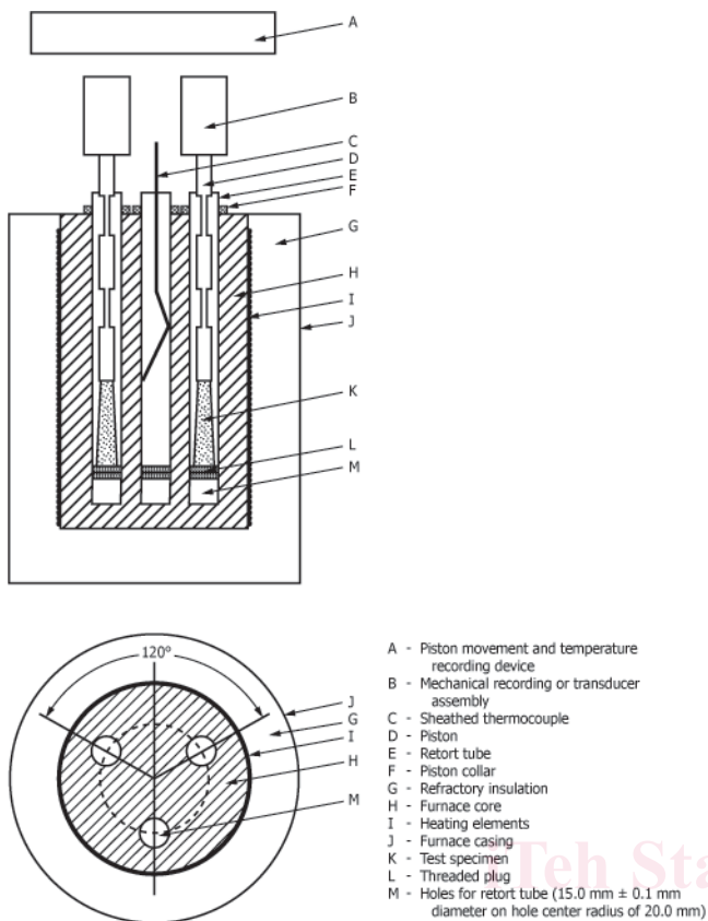
FIG. 2 Typical Dilatometer Apparatus
