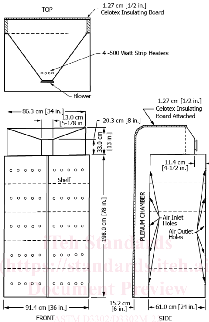
FIG. 2 Air-Drying Oven
