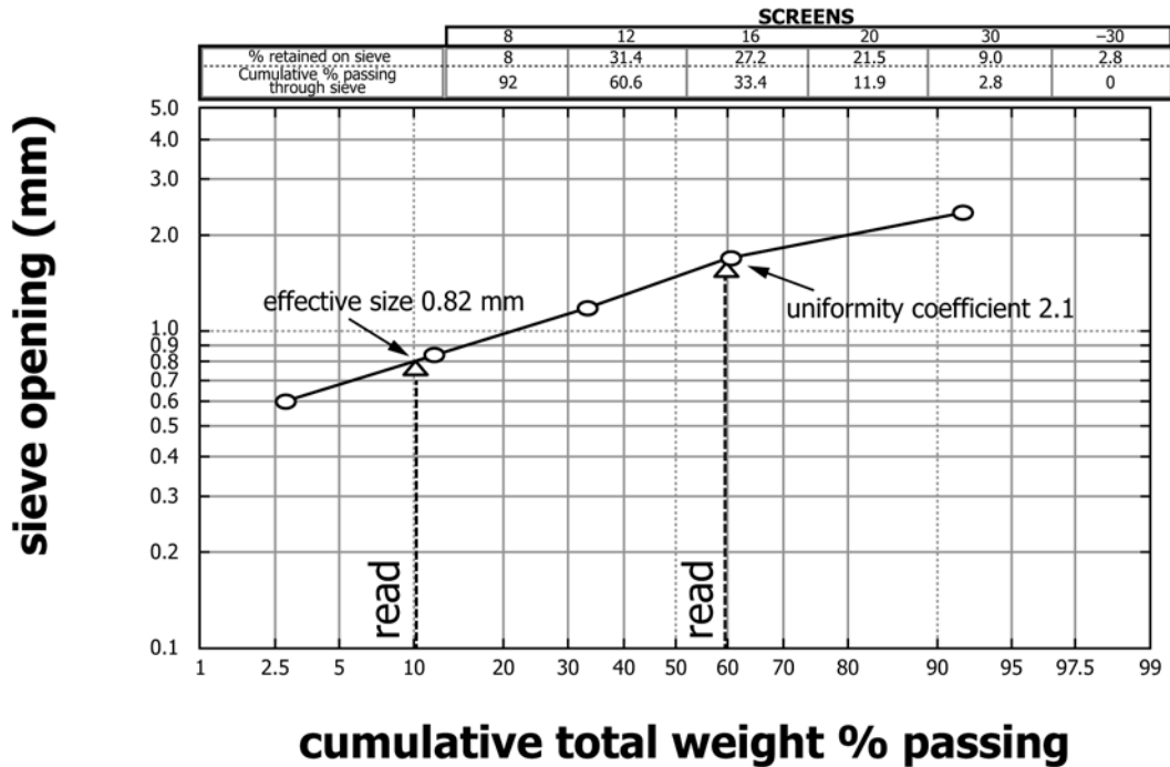
FIG. 1 Cumulative Particle Size Distribution Curve
