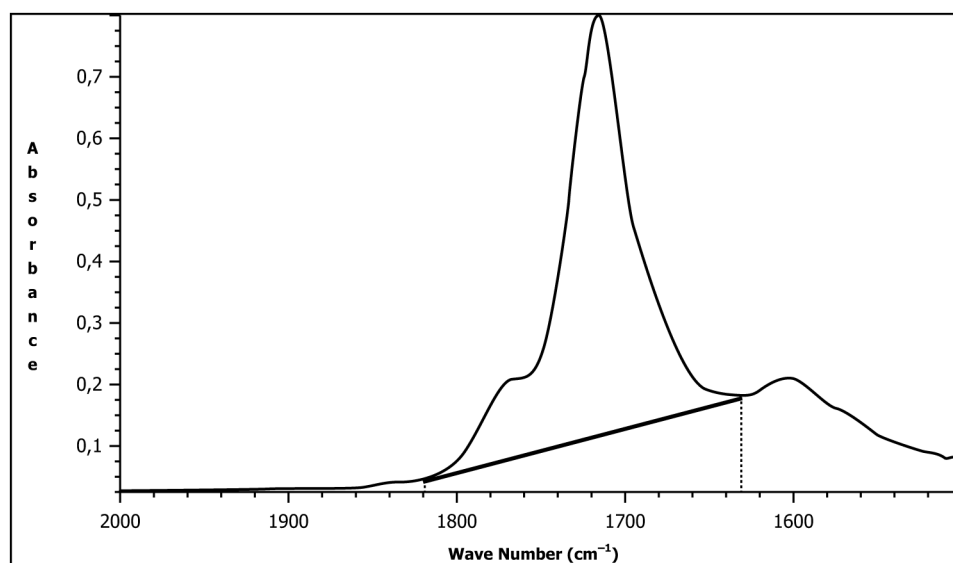
FIG. 1 Area of Spectrum Showing the Result of the Subtraction of Aged Oil Spectrum and Fresh Oil Spectrum
