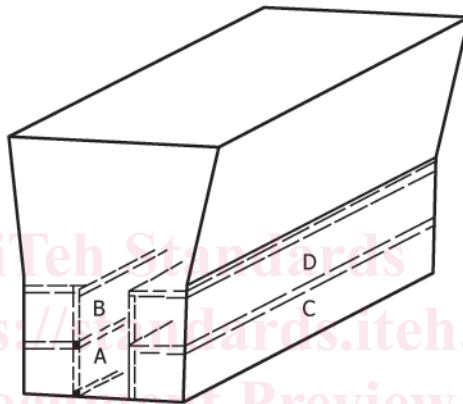
(c) 3-in. [75-mm] Y-Block—Four blanks for 0.50-in. [13-mm] diameter tension test specimens.
