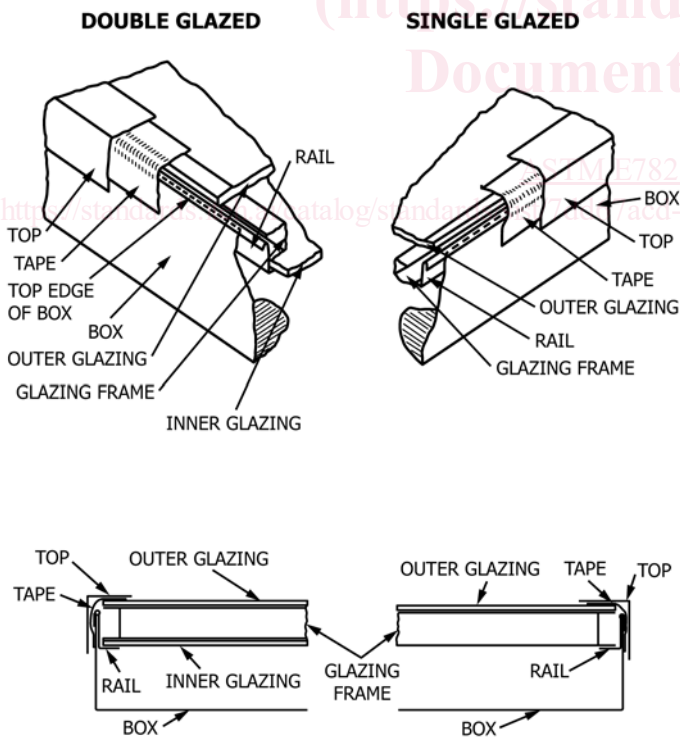
FIG. 5 Natural Weathering Box Assembly—Rigid Glazing
