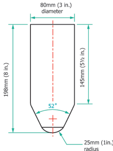
FIG. 5 Weight Outer Dimensions
