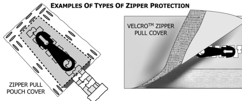
FIG. 5 Examples of Zipper Protection
