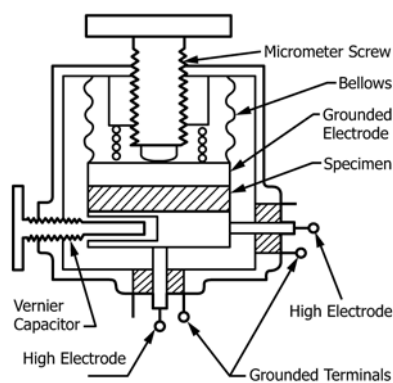
FIG. 9 Micrometer-Electrode System
