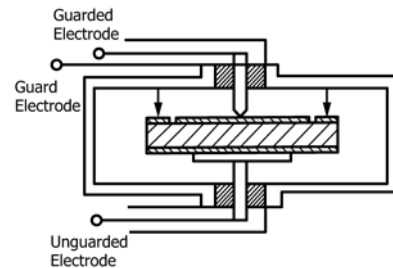
FIG. 8 Three-Terminal Cell for Solids
