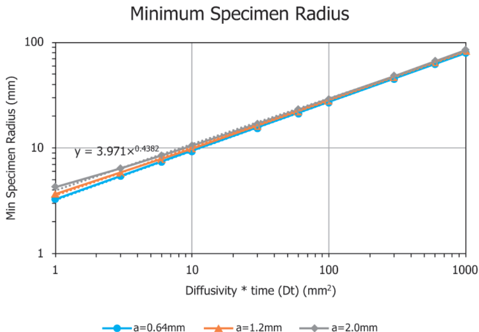
FIG. 1 Minimum Radius of a Specimen
