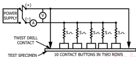
FIG. 2 Diagram of Connections for Contacts and Resistors
