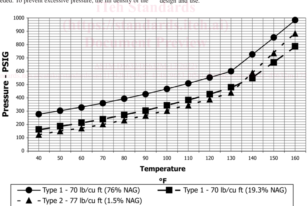
FIG. 1 Isometric Diagram for Bromotrifluoromethane
