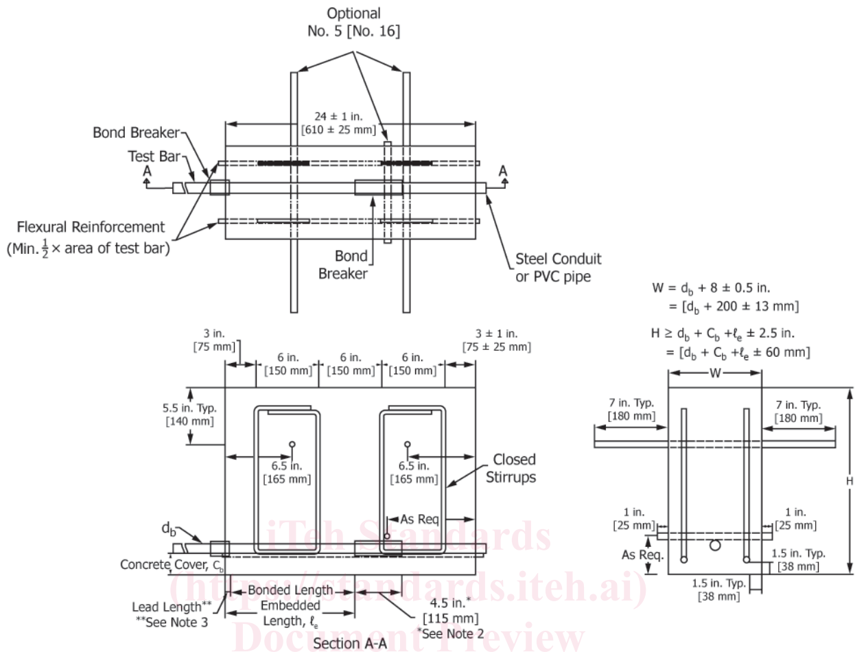
FIG. 2 Beam-End Test Specimens in Casting Position
