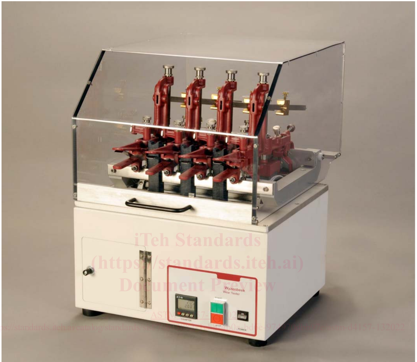
FIG. 1 Oscillatory Cylinder Abrasion Tester
