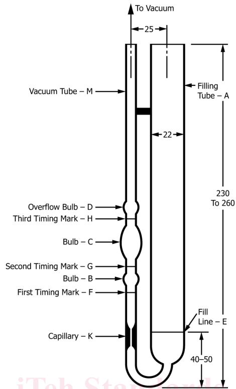
FIG. 2 Cannon-Manning Vacuum Capillary Viscometer
