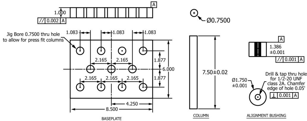
FIG. 6 Drawing of Alignment and Bonding Fixture (inch-pound units)
