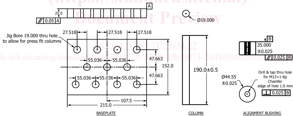
FIG. 5 Drawing of Alignment and Bonding Fixture (SI units)
