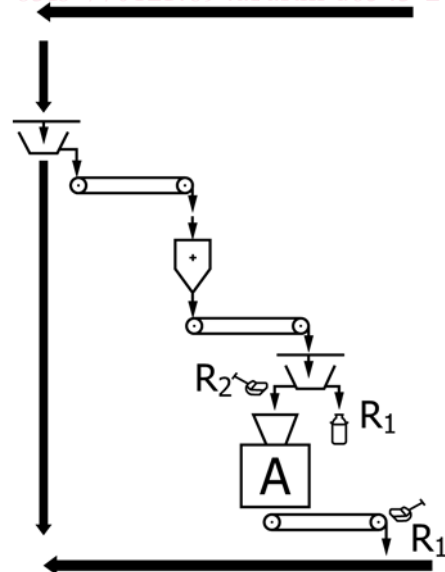
FIG. 3 Analyzer on Secondary Reject—Two-Stage Mechanical Sampling
