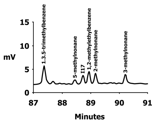
FIG. 8 I17 (unknown)/1,2-methylethylbenzene
