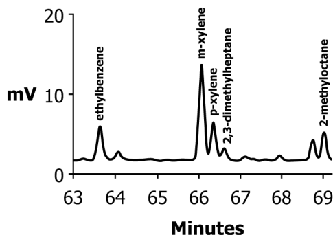
FIG. 7 p -xylene/2,3-dimethylheptane
