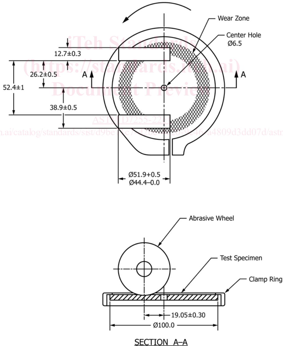
FIG. 2 Arrangement of Rotary Platform Abraser Test Set-up
