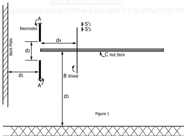
d1 = 24 in. (0.61 m), distance from the wall (back plate) to the arc electrodes d2 = 6 in. (0.15 m) (gap) between electrodes d3 = 53 in. (1.35 m), parallel distance of the hot stick or the racking rod above the floor d4 = 24 in. (0.61 m), distance of the shield from the electrodes d5 = 4 in. (0.10 m), vertical distance between centers of S'1 and S'2 S'1 and S'2 = 24.5 in. (0.62 m), approximate horizontal distance of the sensors from the electrodes S1, S2, S3, S4, S5, and S6 are located vertically, and S1 is 5 ft (1.52 m) from the arc center
