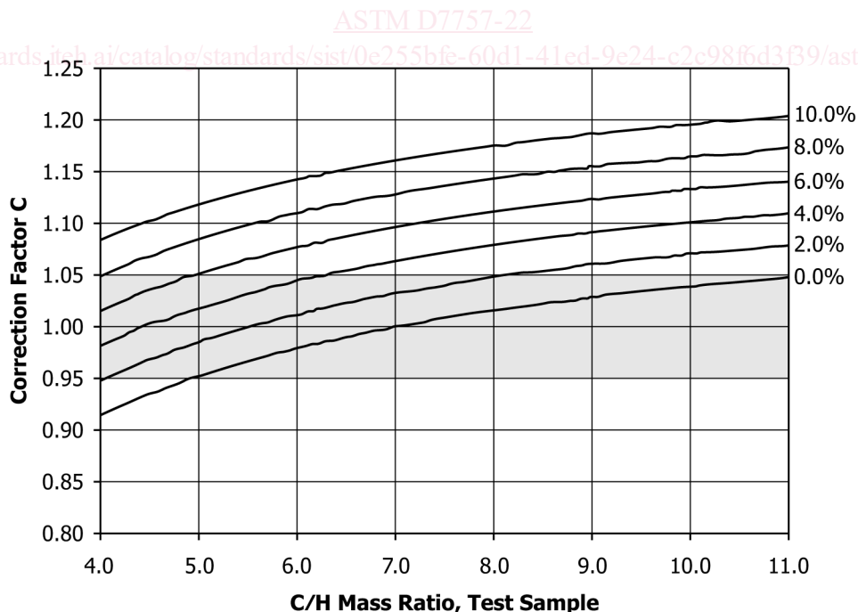
FIG. 2 Matrix Correction for a Test Sample versus C/H and Total Oxygen Content Using Chromium K\alpha for the Excitation Beam
