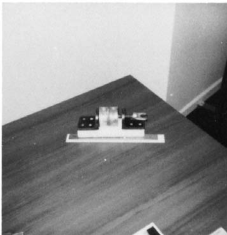
FIG. 1 Cell for Volume Resistivity With Electrodes Made With Metal Foil, Conductive Paint or Similar High Conductivity Material as Described in Test Method D257
