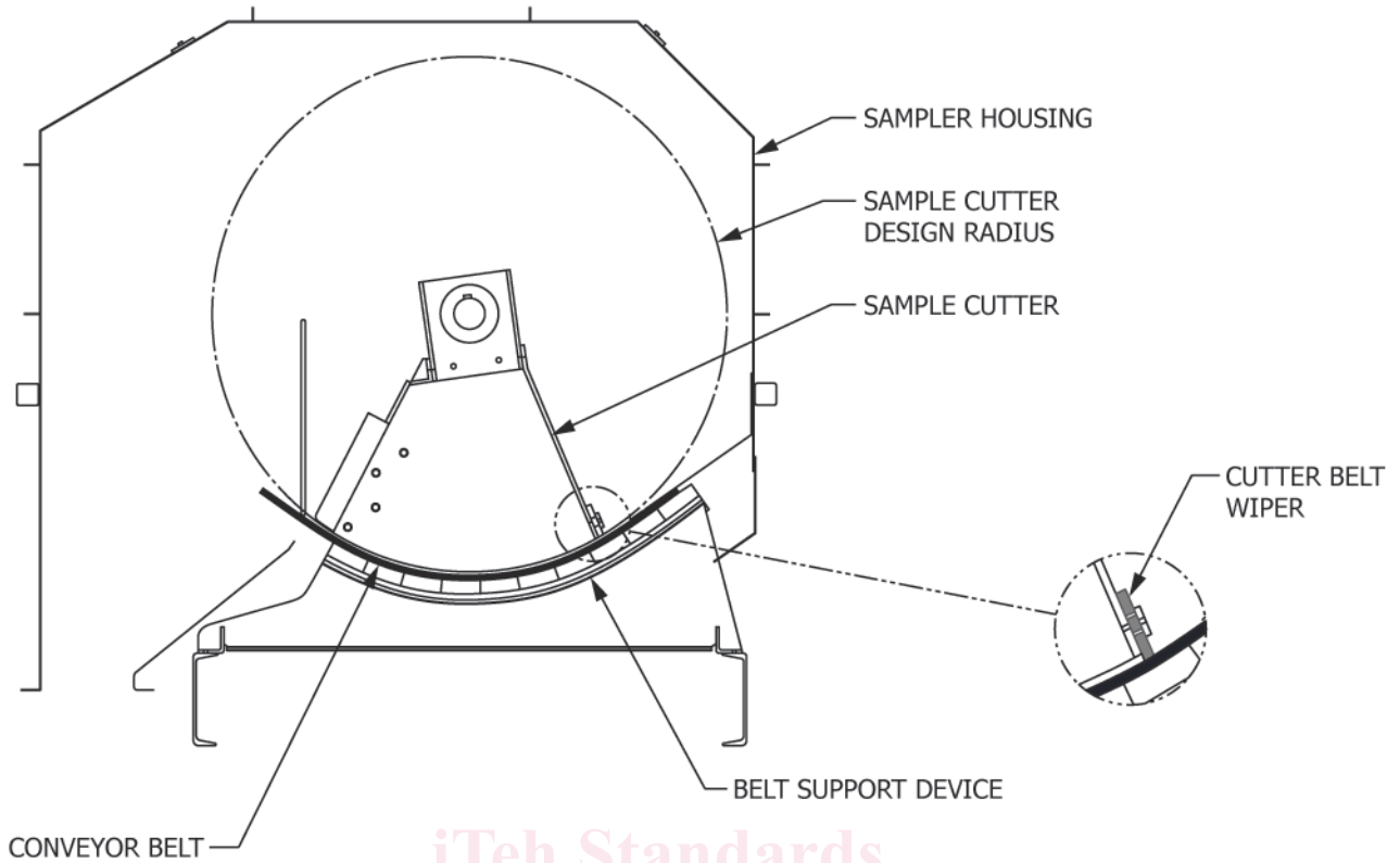
FIG. 2 Cross Belt Sampler With Conveyor Arc Support
