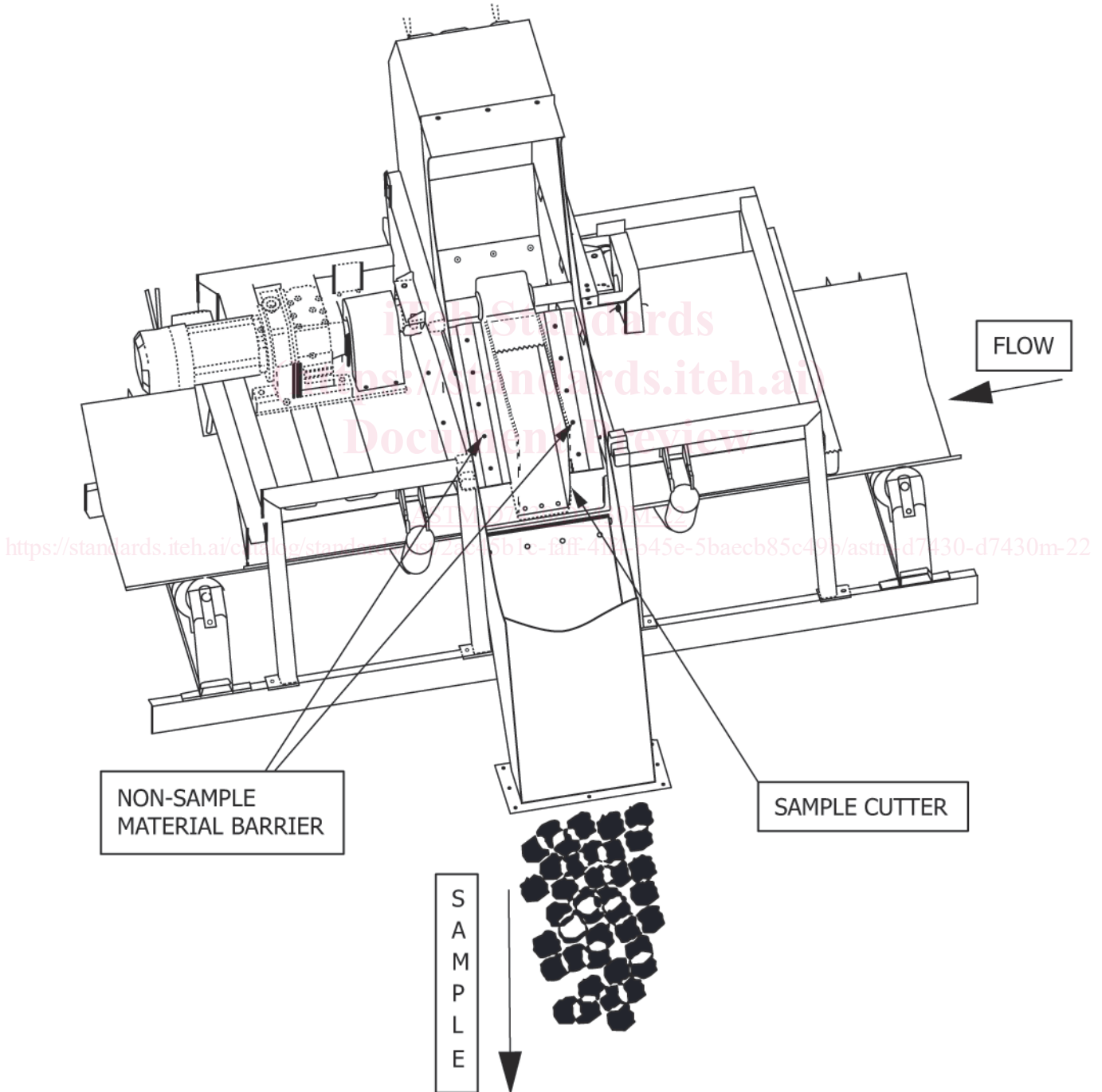
FIG. 4 Cross-Belt Sampler
