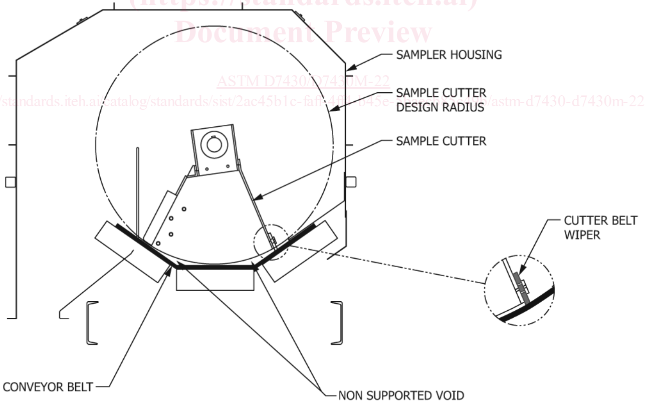
FIG. 3 Cross-belt Sampler Without Conveyor Arc Support
