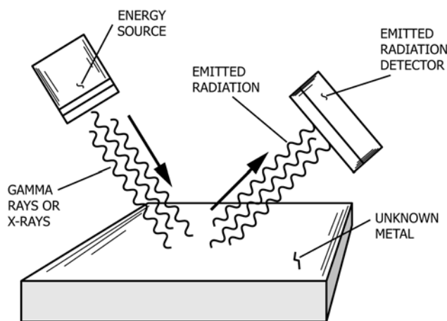
FIG. 1 X-Ray Fluorescence Spectrometry
