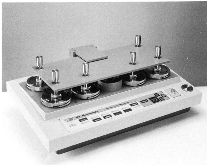
FIG. 1 Martindale Abrasion-Tester
