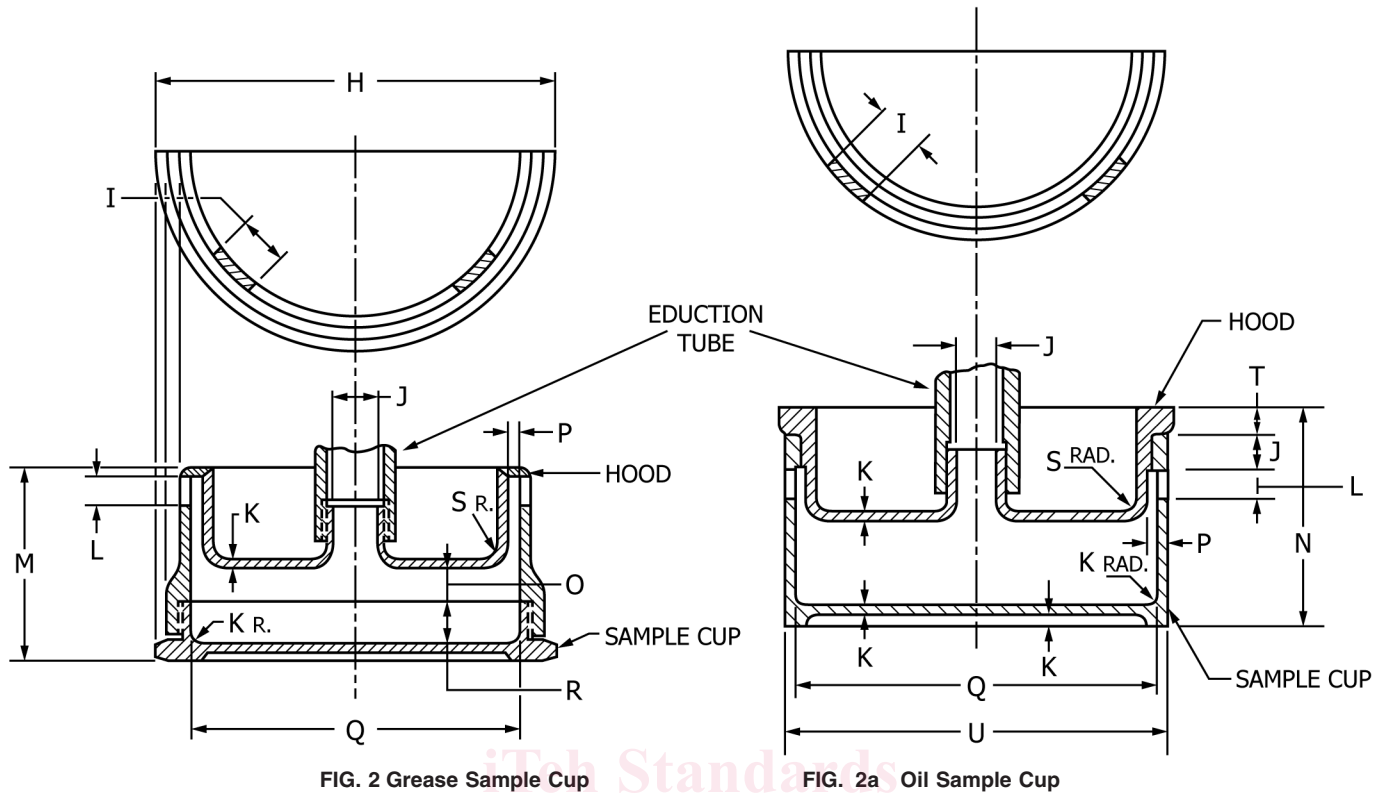
FIG. 2 Grease Sample Cup
