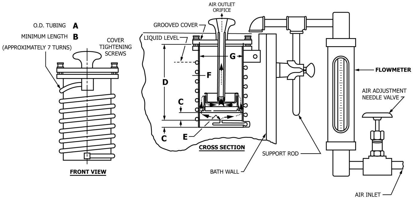
FIG. 1 Evaporation Test Cell
