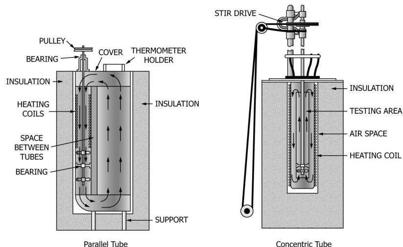
FIG. 1 Alternative Designs of Top Stirred Comparison Baths Without Controllers-Controllers
