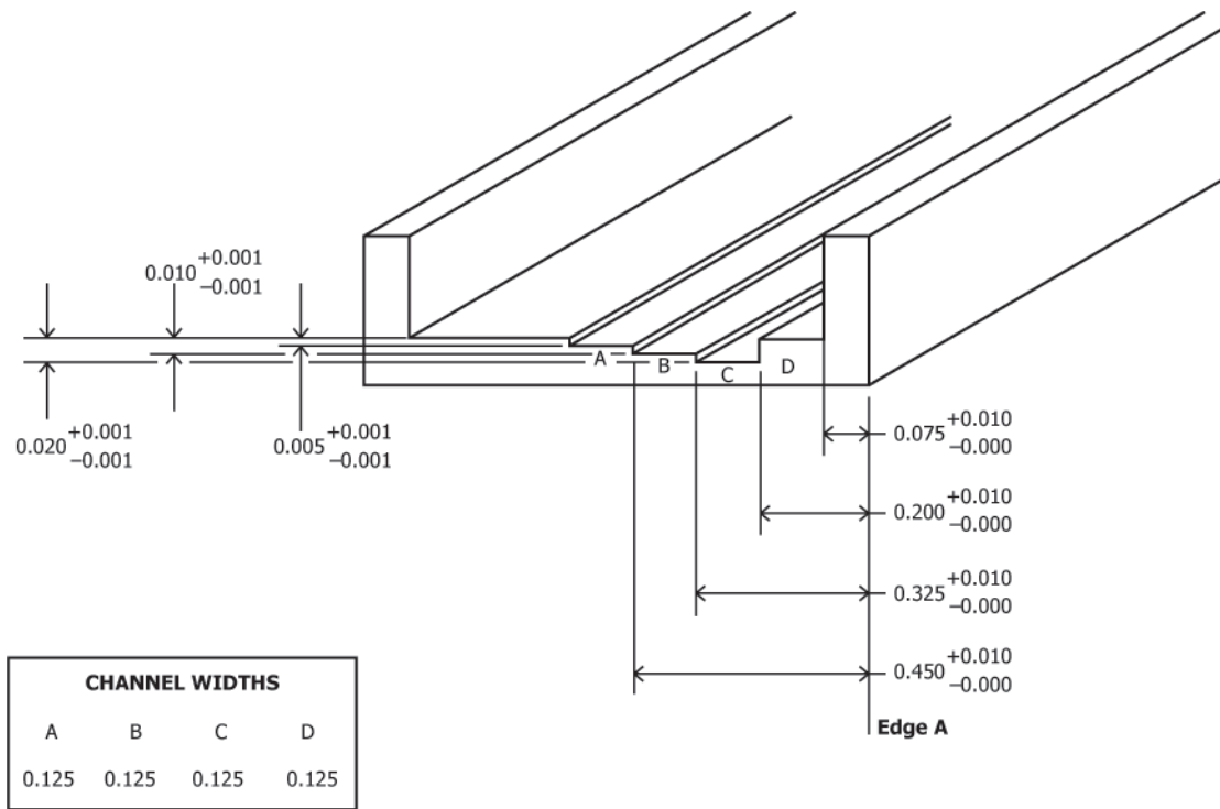
FIG. 3 Channels A Through D in Main Channel
